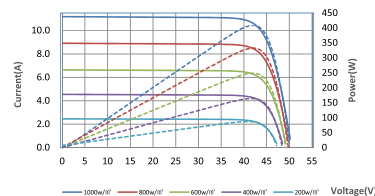
Current-Voltage Curve (BSM455M-72HPH)
